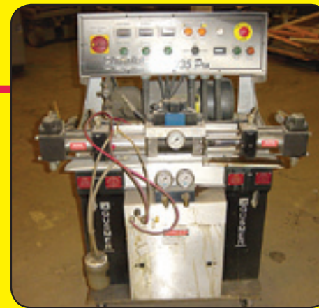
Gusmer H-20/35 Proportioner/Impingement Gun System
